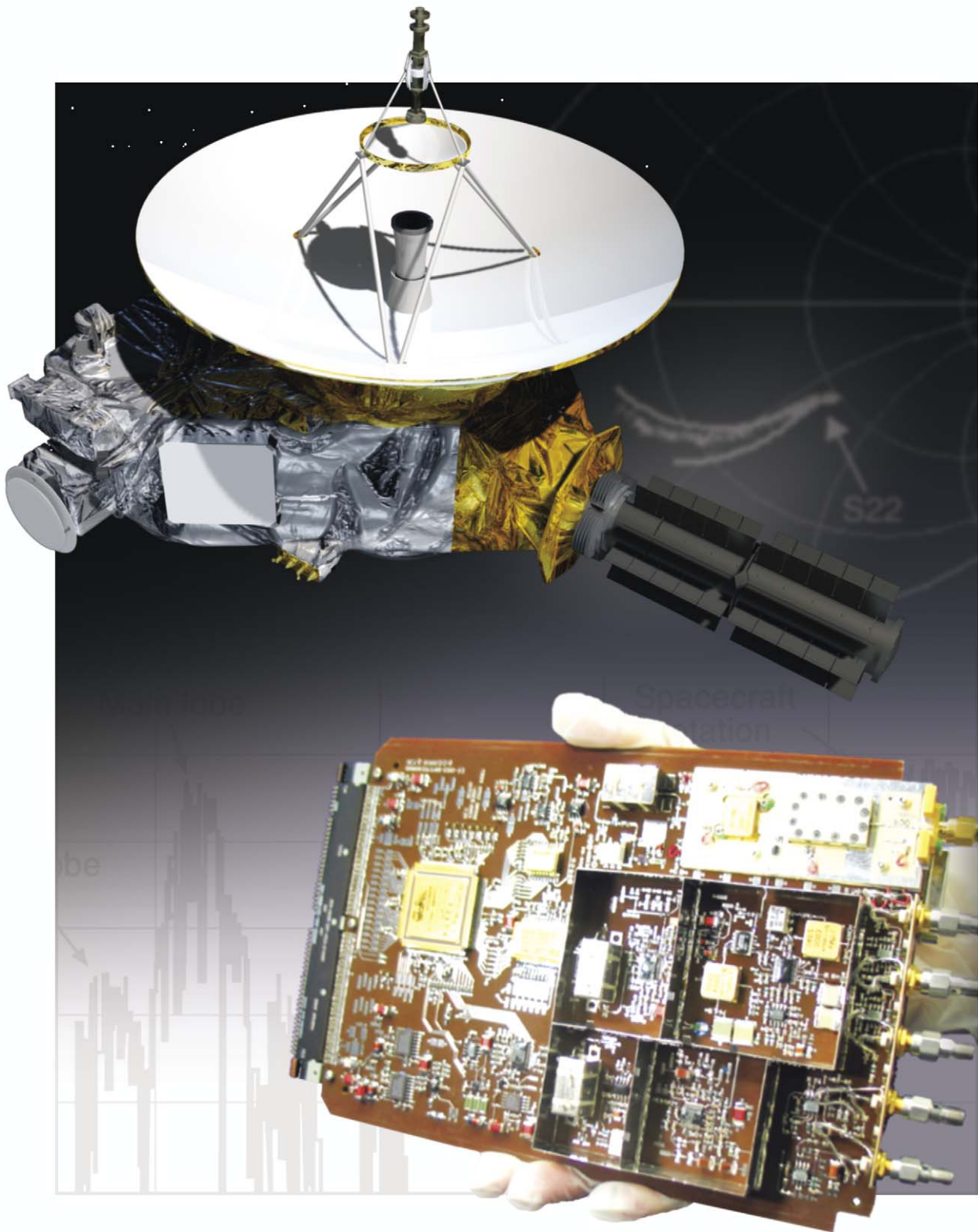
The radio communication system for the New Horizons Pluto flyby mission is challenging due to the extreme distance involved and the limited power available on the spacecraft. These challenges have been met with a high gain antenna that operates at cryogenic temperatures (top) and a low-power, ultrastable receiver system for communications and navigation (bottom).
